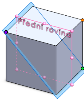
Planes directed through element are derived from basic plane
