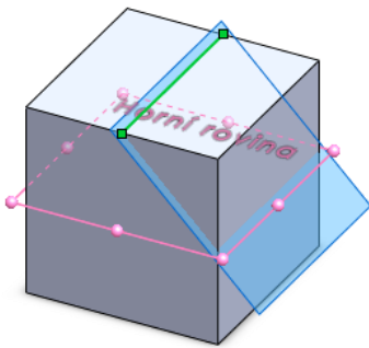
Inclined plane under angle to auxiliary sketch
